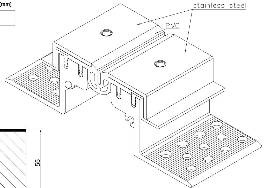
CONECTO GA 43.10.55 S VIEW
